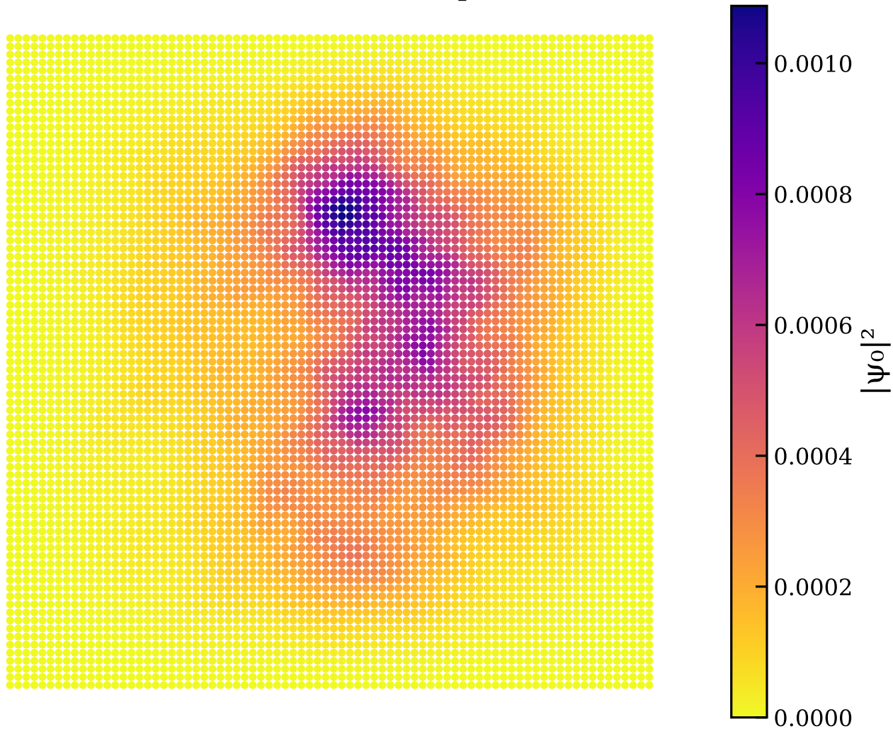
Ground state distribution: Square 80x81
